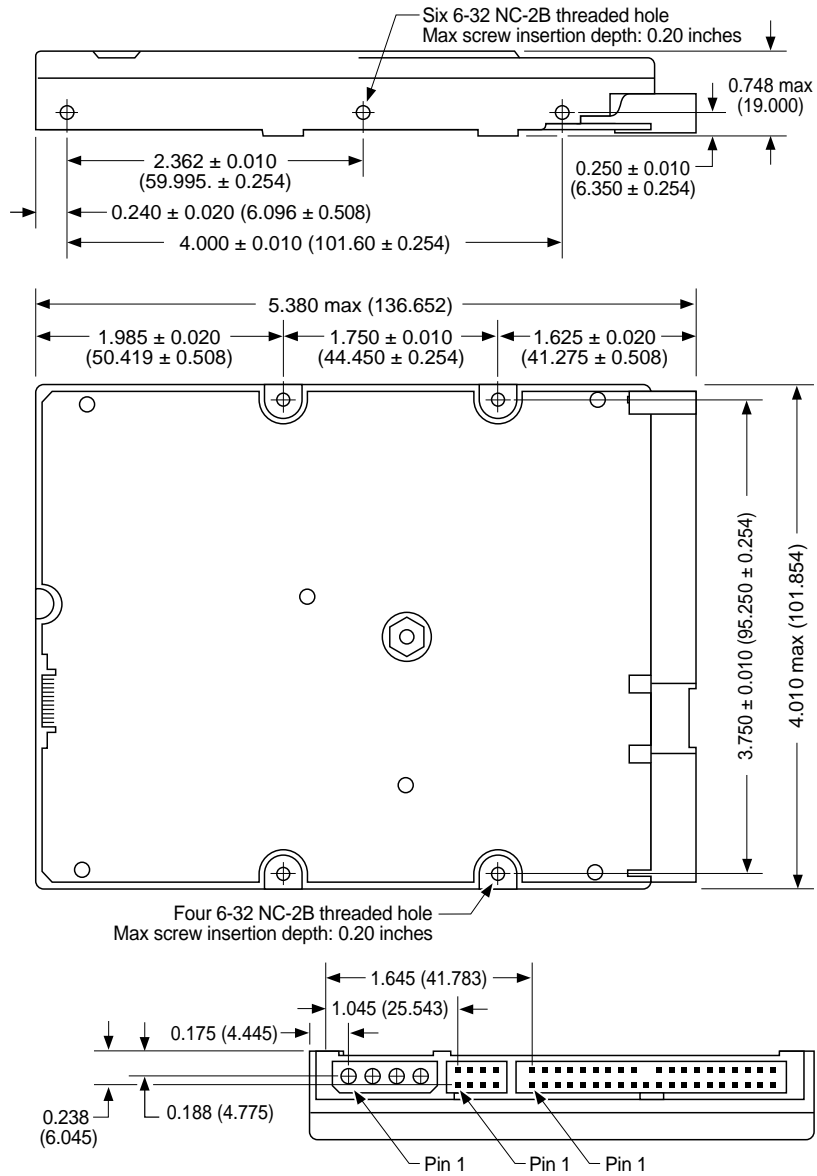
Figure 6. Mounting dimensions
